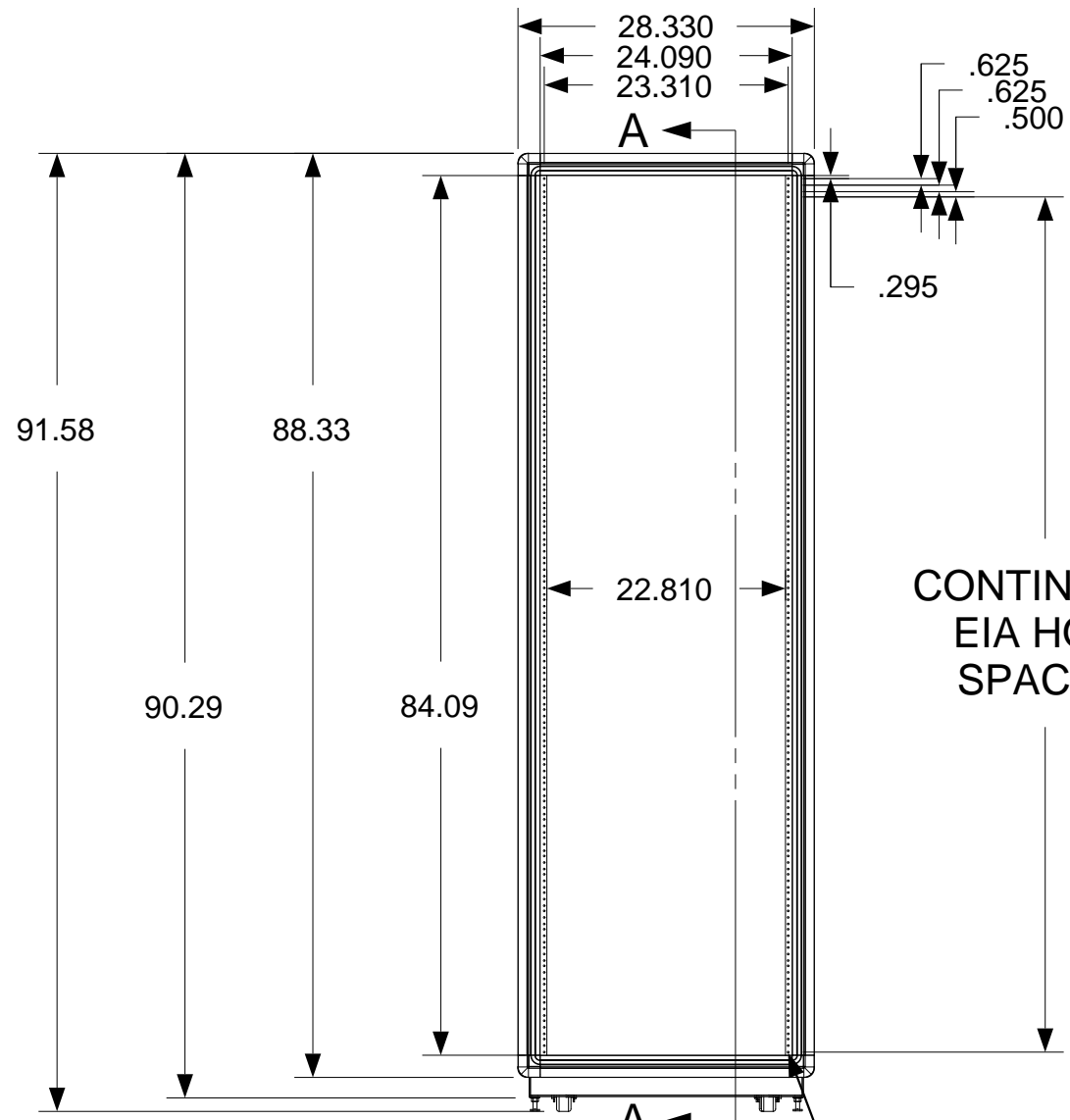
FRONT VIEW
