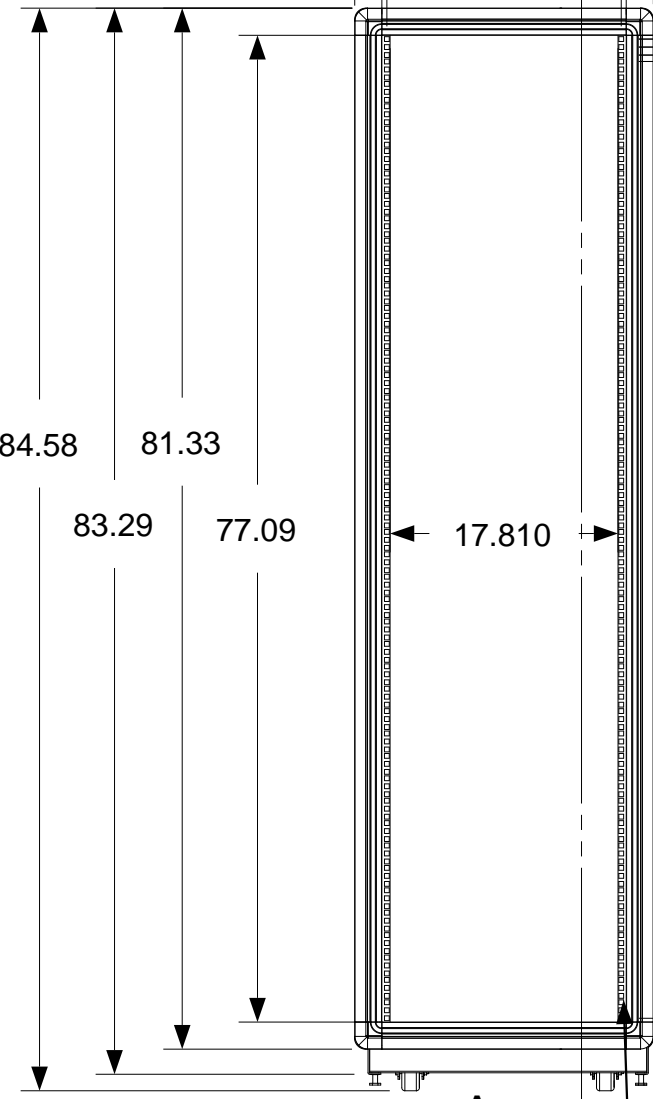
FRONT VIEW
