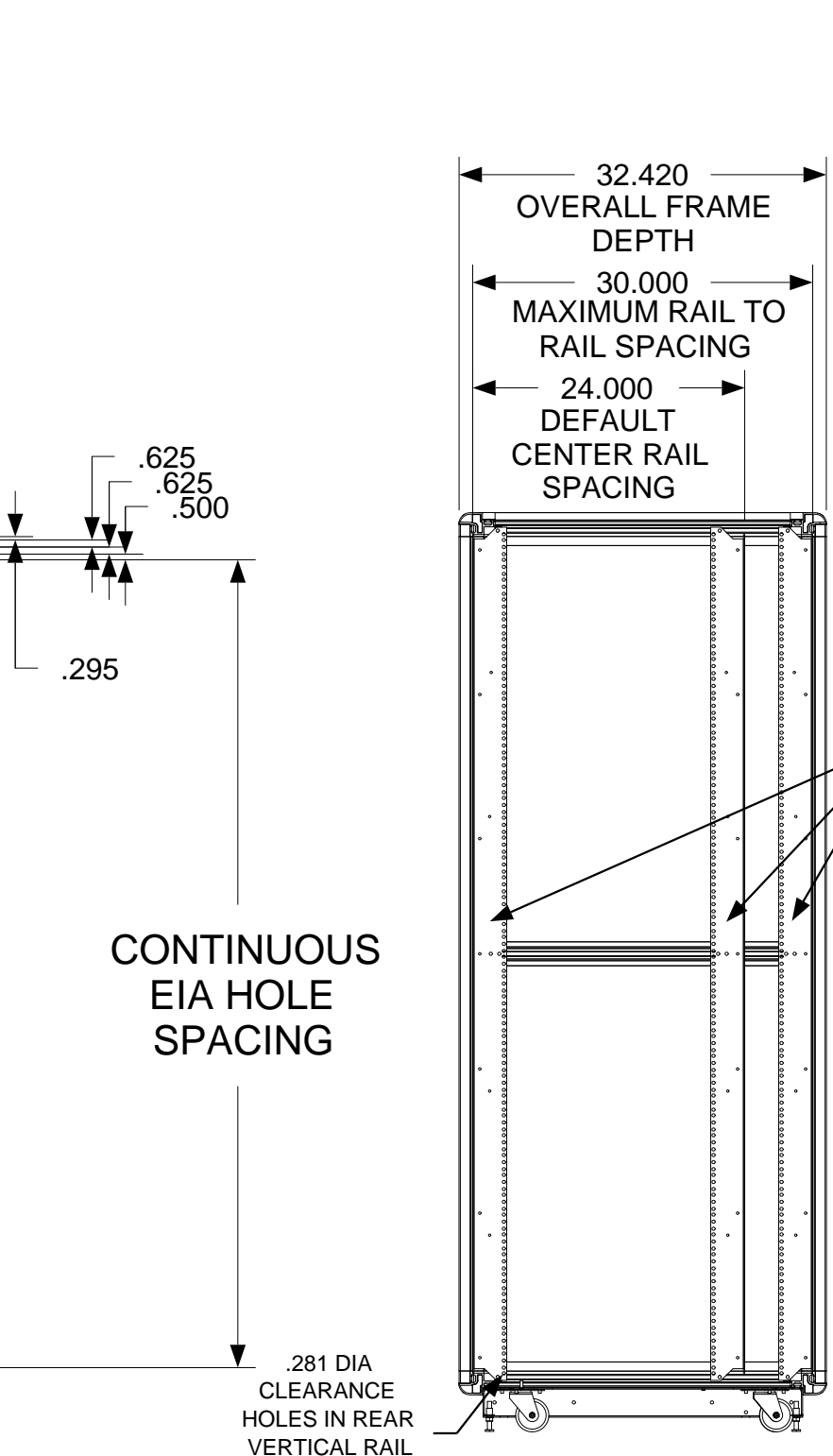
SIDE SECTION VIEW
