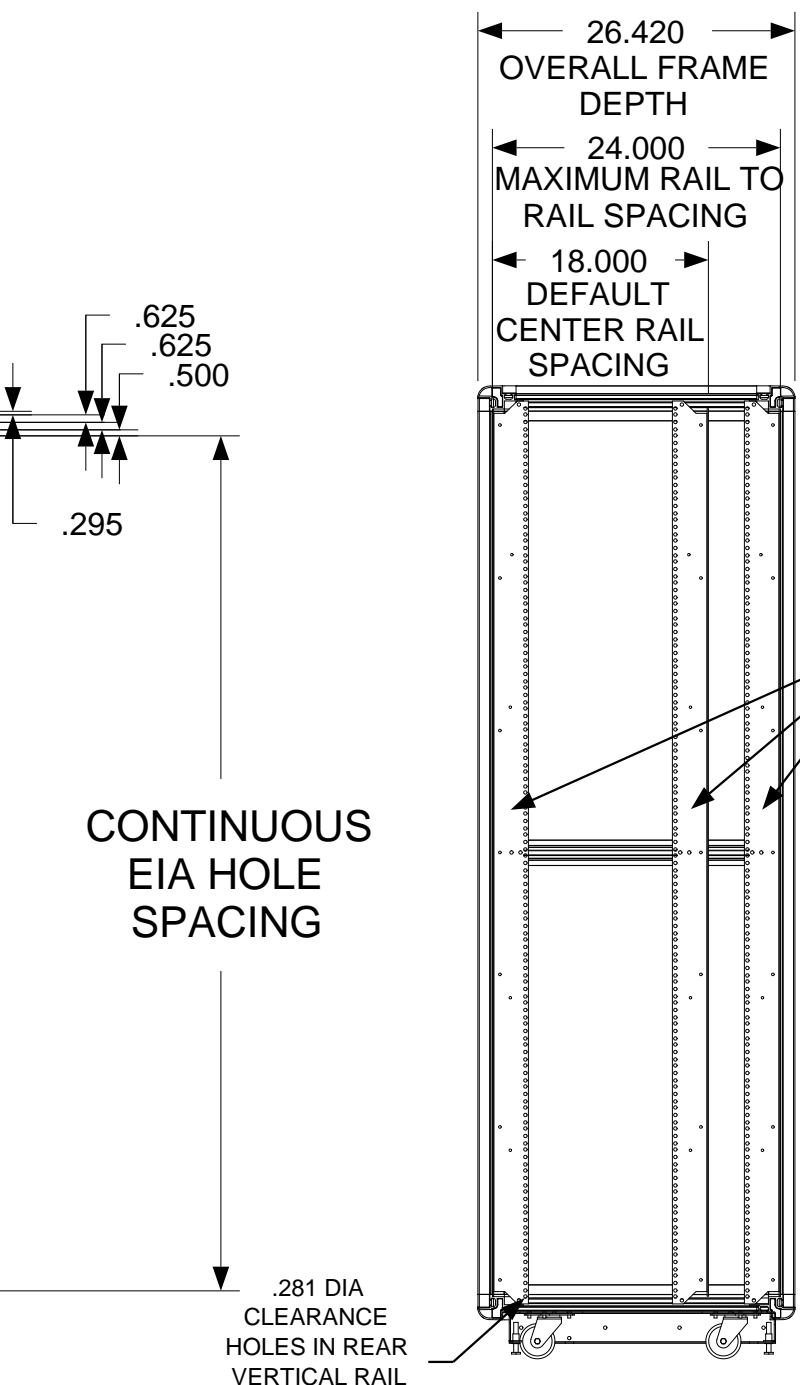
SIDE SECTION VIEW
