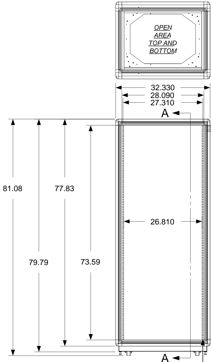
FRONT VIEW
