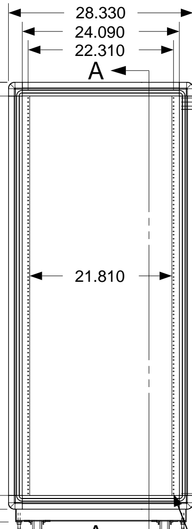
FRONT VIEW
