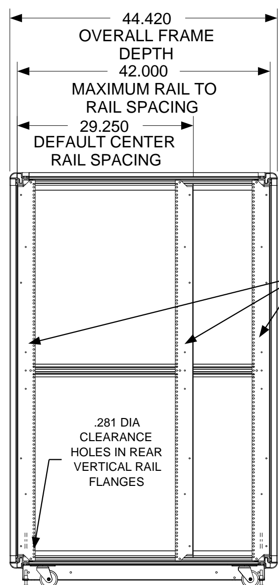
SIDE SECTION VIEW
