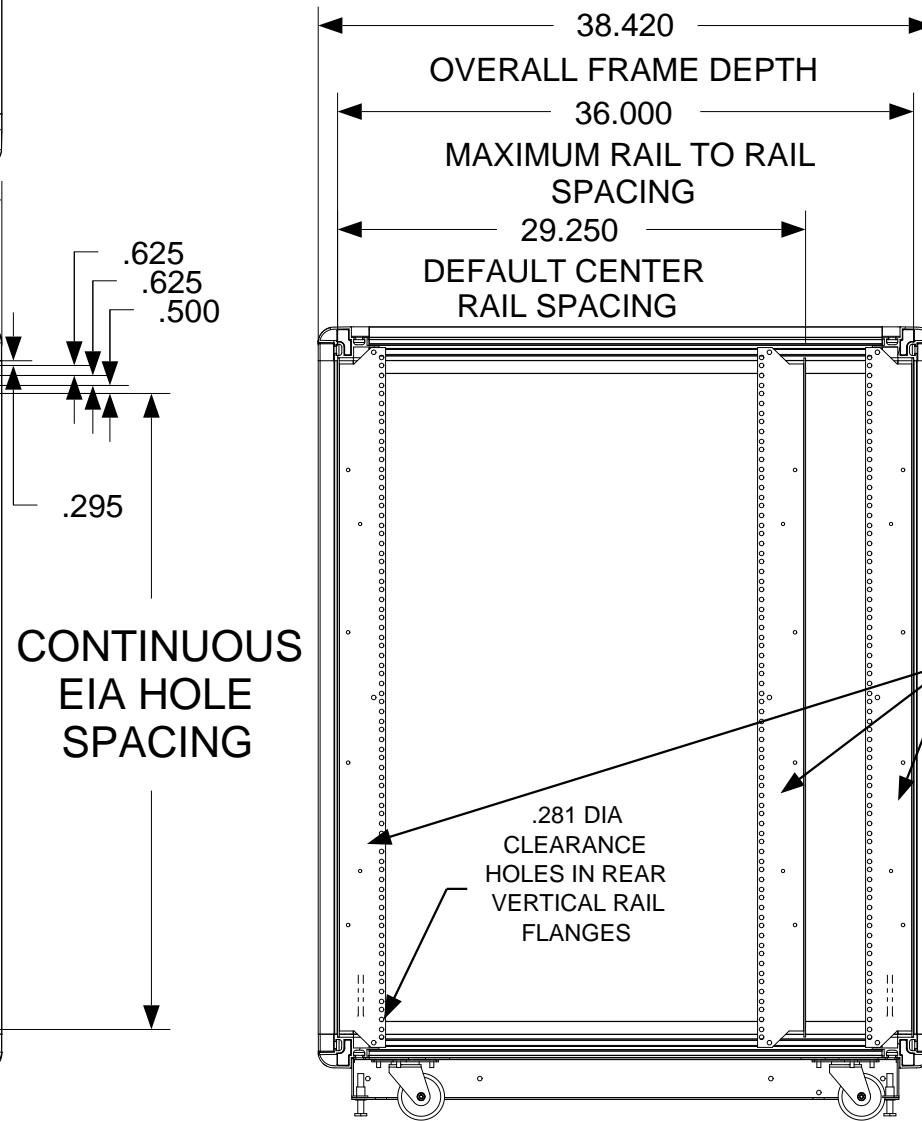
SIDE SECTION VIEW
