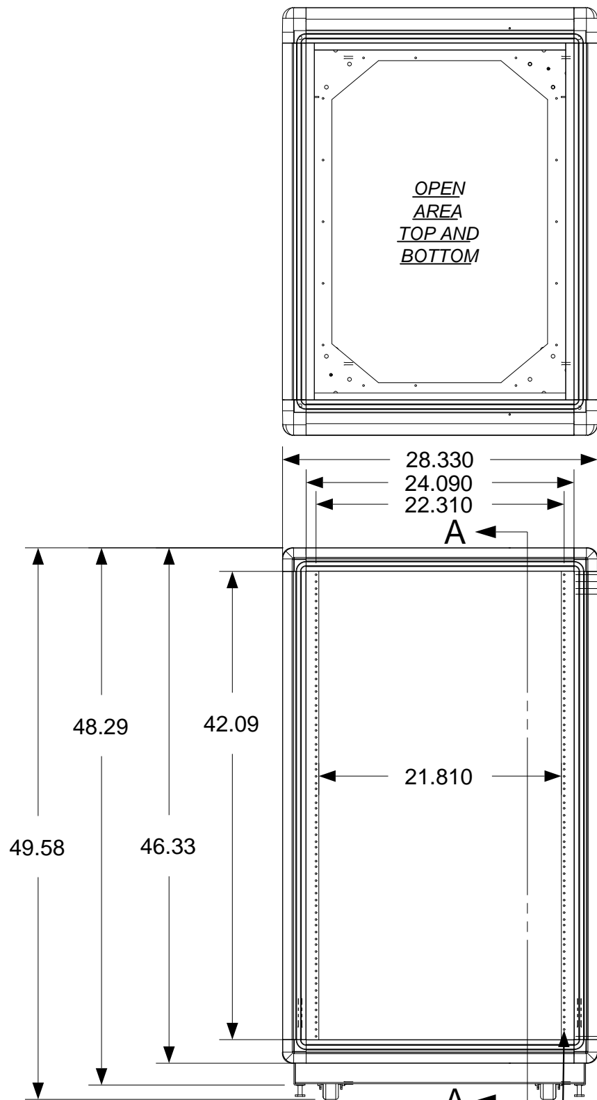
FRONT VIEW
