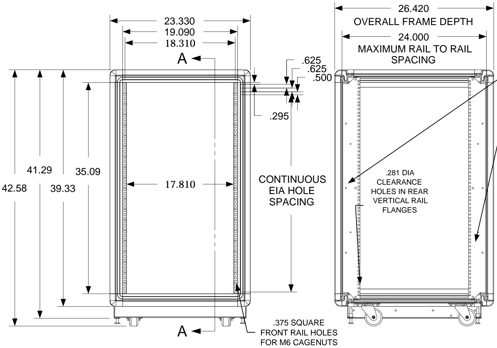
FRONT VIEW
